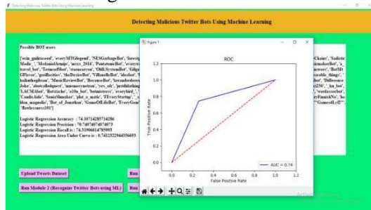
Fig.7: ROC graph
