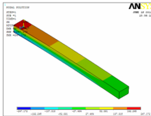
Fig. 5 Vonmises Stress
