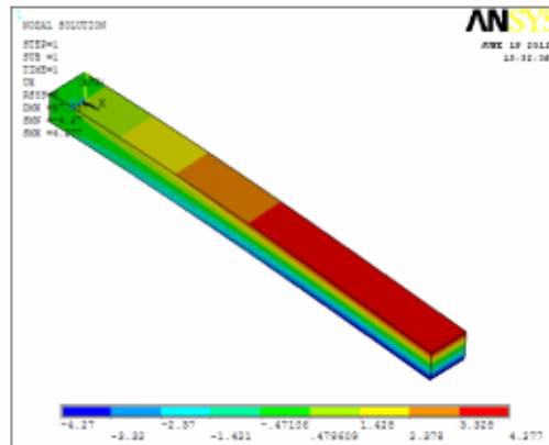
Fig. 4 Total Deformation
