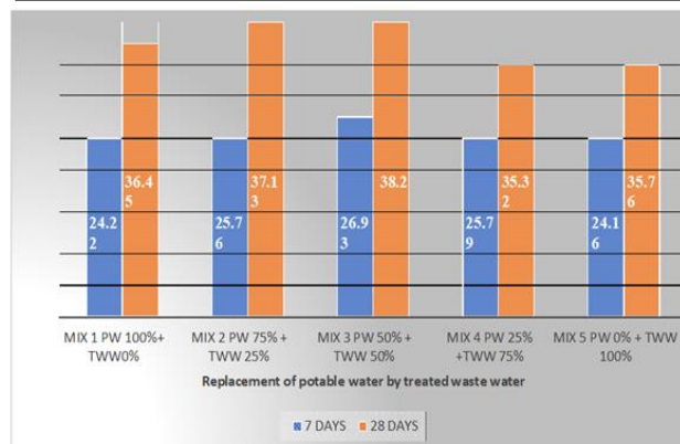
Graph 5.4.compressive strength of concrete
