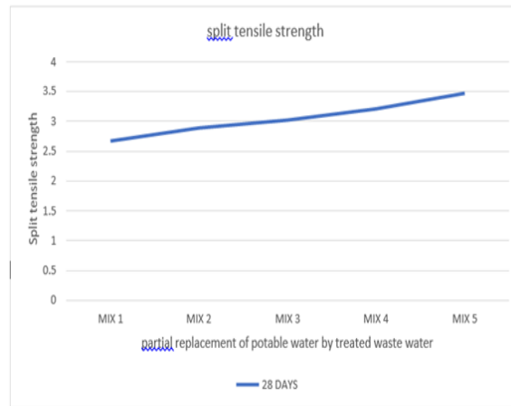
Graph 5.5 split tensile strength of concrete
