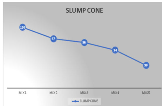
Graph 5.1 slump cone test results
